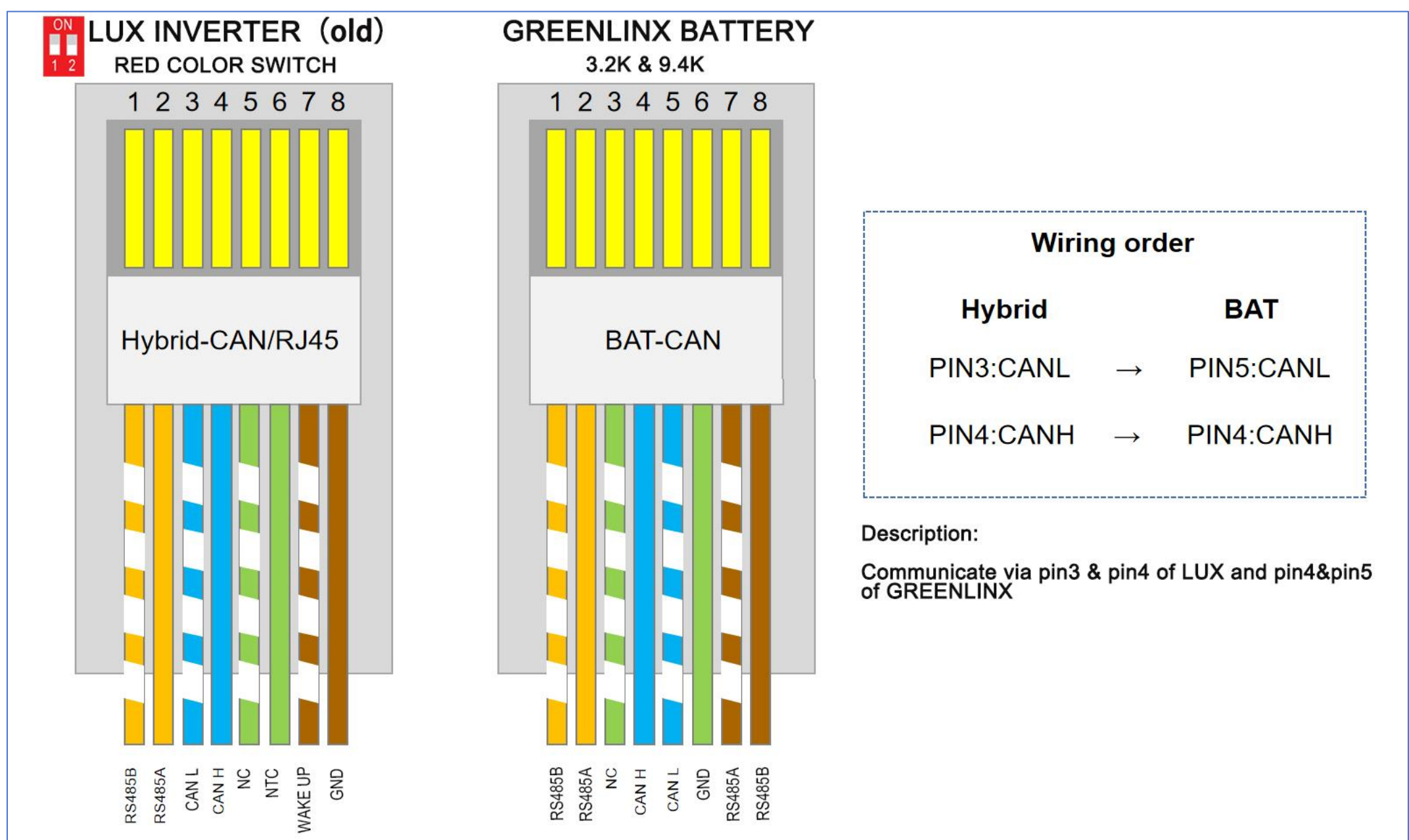
Picture 2: Schematic wiring diagram of LUX(old) and GREENLINX
