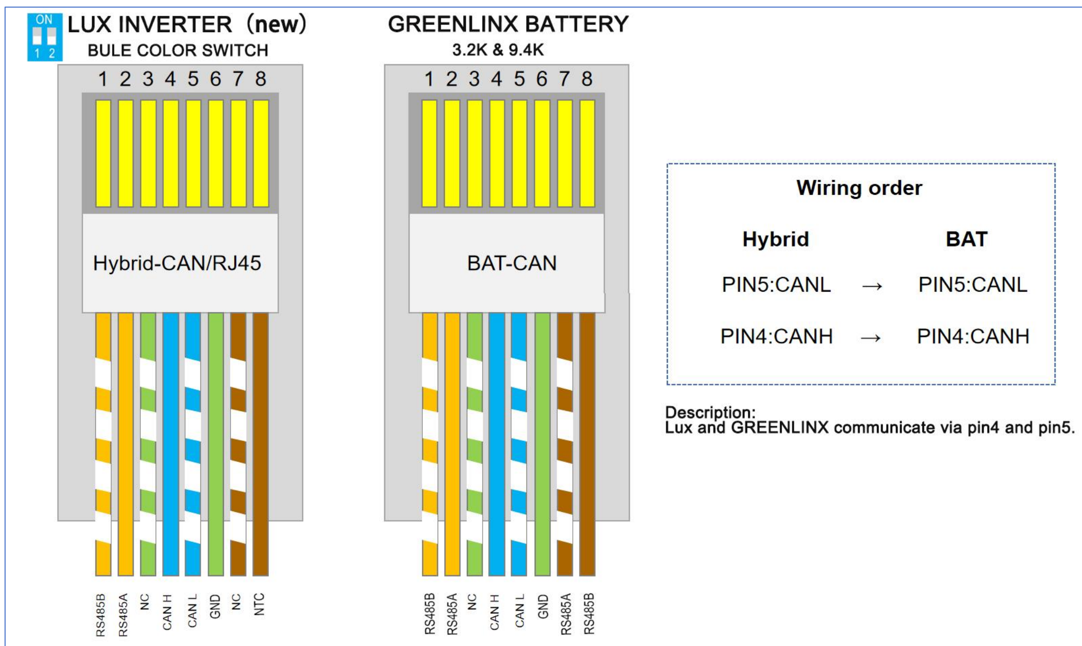
Picture 1: Schematic wiring diagram of LUX(new) and GREENLINX
