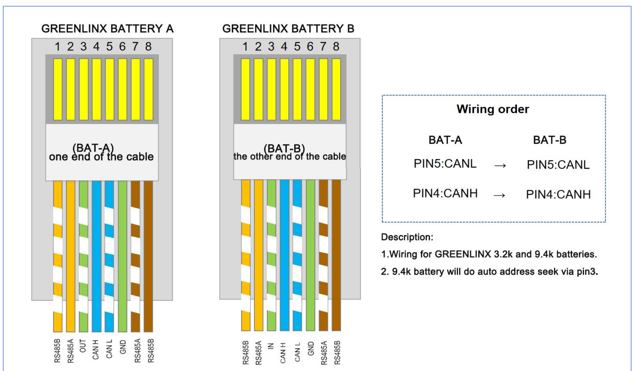
Picture 3: Schematic wiring diagram of GREENLINX batteries.(For 3.2k and 9.4k)
