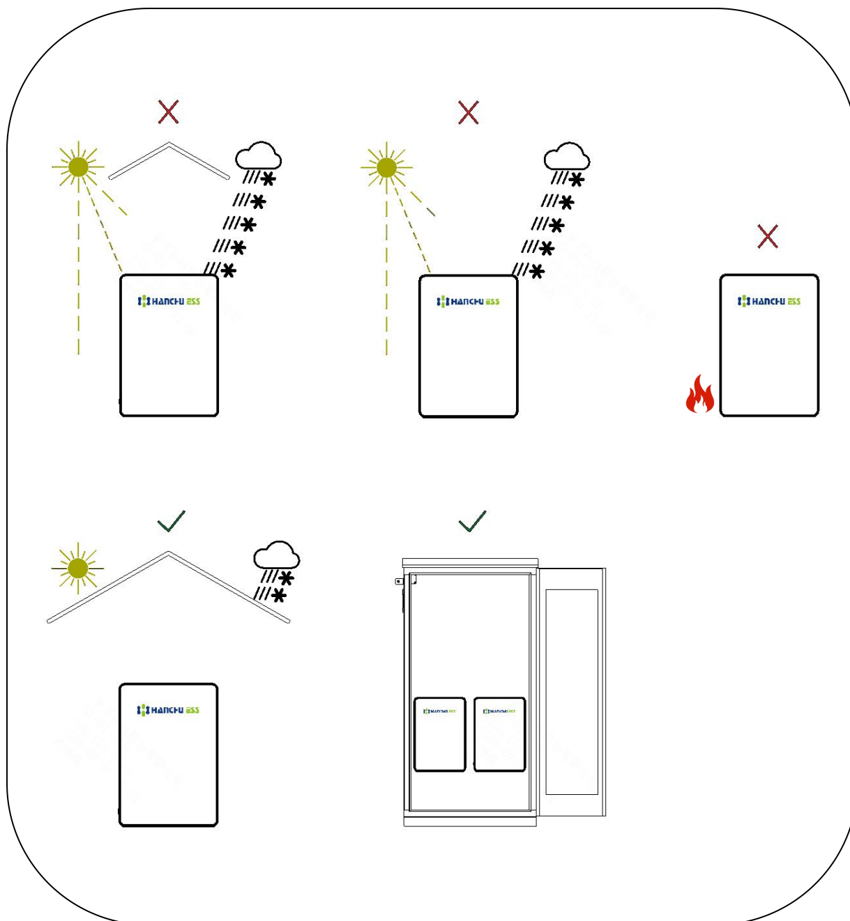
Figure 4 Installation Environment
