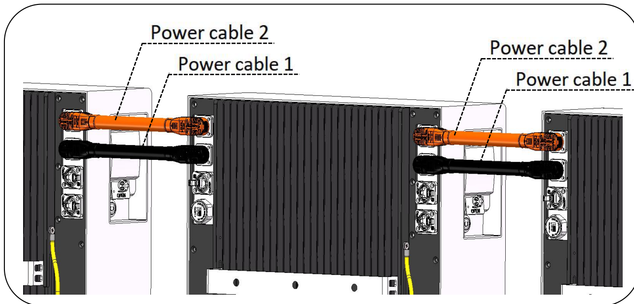
Figure 15 Sample of Connection for the Power Cable 1-2
